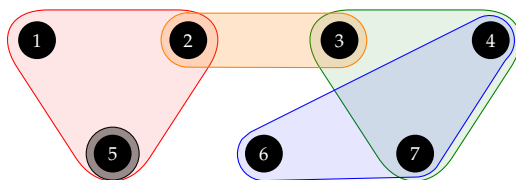
Figure 1.1: A hypergraph on [7] .
